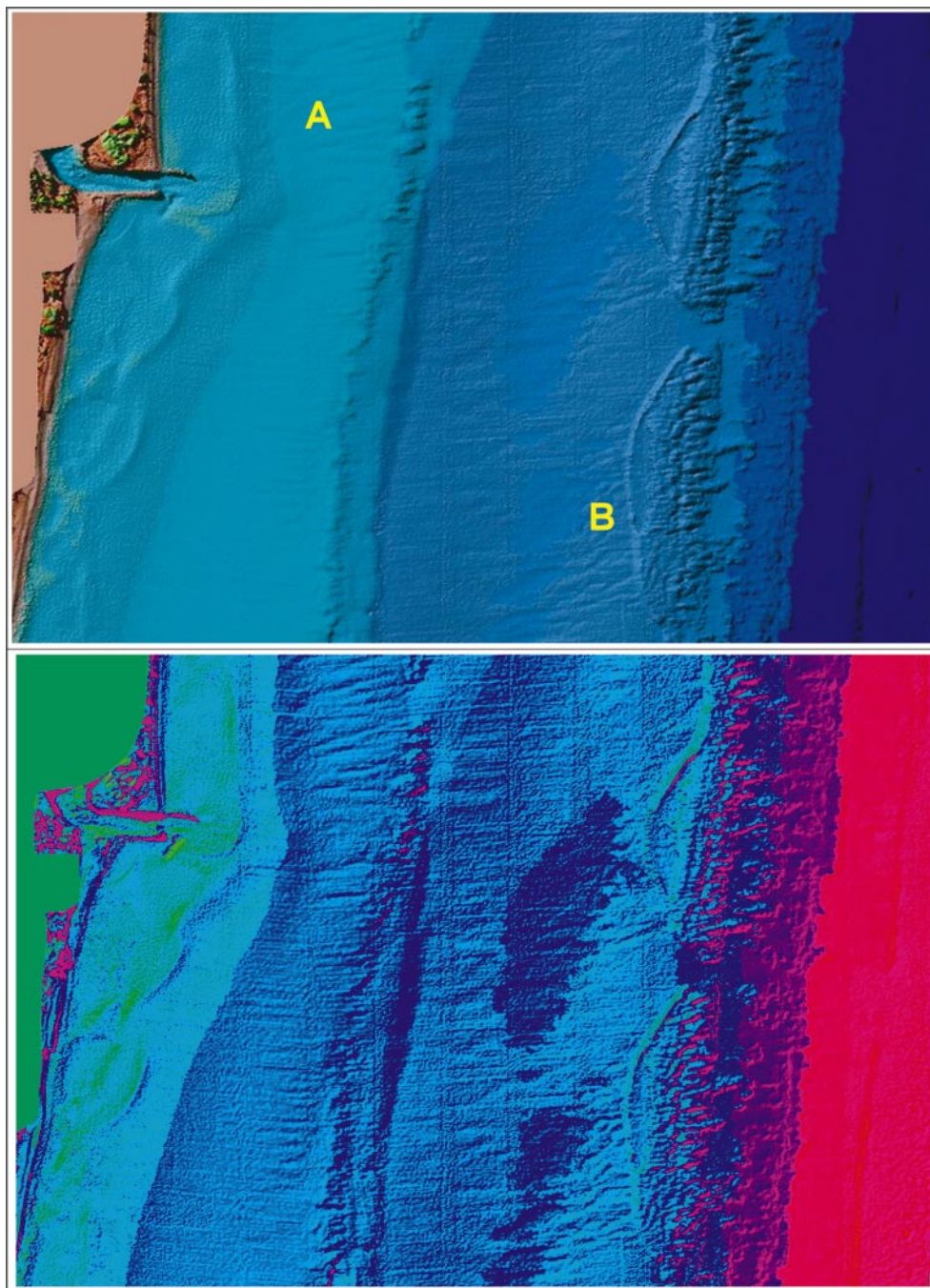
Figure 4. Enhanced false-color imagery of seafloor features offshore the Boca Raton Inlet. The highpass-filtered (upper) image was subjected to a gradient filter technique that emphasizes changes in DN numbers over a specified number of pixels. This kind of “change in slope” image combines some classes separated in previous images but discerns bathymetric change. Note in particular how close-order depth differences are highlighted in the forereef spur-and-groove topography (right side of lower image, where reddish hues for deeper water transect bluish hues for shallower water) and how clearly diabathmic ridges and troughs stand out for nearshore and inter-reefal sands.
