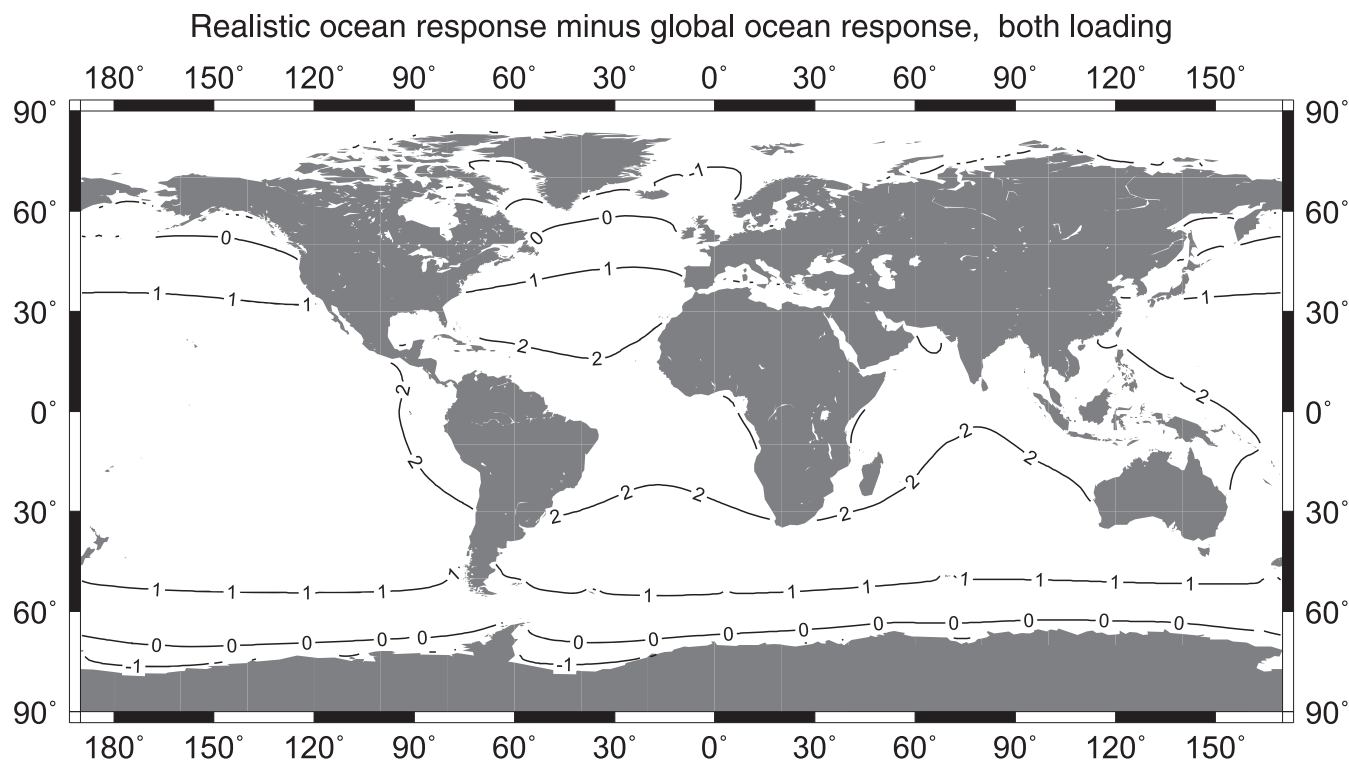
Figure 2. Reproduction using a 1° grid of Figure 1 of Agnew and Farrell (1978), showing the self-consistent response of the generic long period with a realistic ocean and loading ( cf. Figure 1) minus what Agnew and Farrell called the equilibrium tide, with a global ocean (no land) and loading. (Nominal units in millimetres.)
