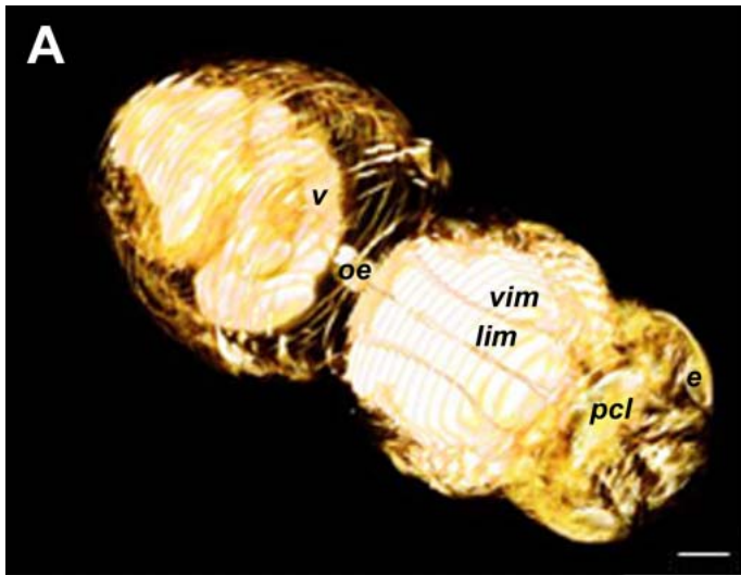
Figure 3. Three dimensional reconstructions of a Vespsula vulgaris queen. A, B and E are based on 59 250 \mu\text{m} MRI slices of a whole wasp (voxel size 31 x 31 x 250 \mu\text{m} , 6 averages, TR 0.5 s, TE 2.6 ms, acquisition time 13 hours); C and D are based on 61 140 \mu\text{m} slices of a wasp abdomen (voxel size 28 x 28 x 140 \mu\text{m} , 6 averages, TR 0.5 s, TE 2.6 ms, acquisition time 13 hours); all are in orthogonal perspective, scale bars are 1 mm. A (Above) Top view. B (Right) Lateral view with ovaries and poison gland coloured (maximum intensity projection). C (Right) Anterior to posterior view of the abdomen. D (Right) Ventral view of the abdomen (data set interpolated from 61 to 256 slices using the Lanczos method). E (Page 8) Facial view of the head.
