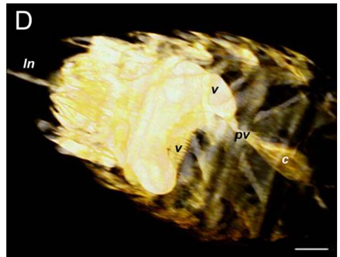
Figure 3. Three dimensional reconstructions of a Vespsula vulgaris queen. A, B and E are based on 59 250 \mu\text{m} MRI slices of a whole wasp (voxel size 31 x 31 x 250 \mu\text{m} , 6 averages, TR 0.5 s, TE 2.6 ms, acquisition time 13 hours); C and D are based on 61 140 \mu\text{m} slices of a wasp abdomen (voxel size 28 x 28 x 140 \mu\text{m} , 6 averages, TR 0.5 s, TE 2.6 ms, acquisition time 13 hours); all are in orthogonal perspective, scale bars are 1 mm. A (Above) Top view. B (Right) Lateral view with ovaries and poison gland coloured (maximum intensity projection). C (Right) Anterior to posterior view of the abdomen. D (Right) Ventral view of the abdomen (data set interpolated from 61 to 256 slices using the Lanczos method). E (Page 8) Facial view of the head.
