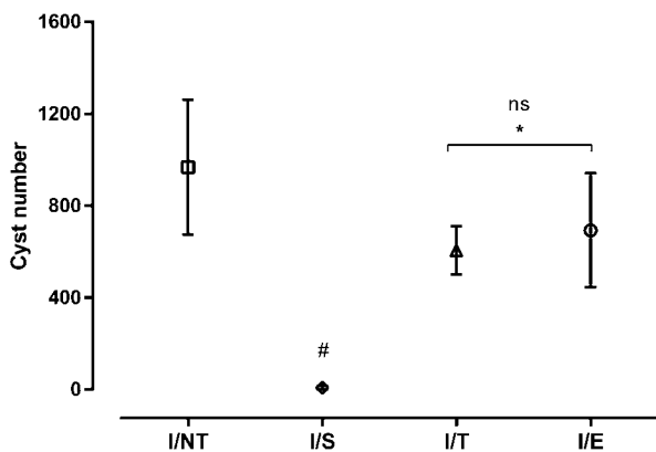
FIGURE 3. Number of brain cysts in C57BL/6 mice orally infected with 10 Toxoplasma gondii ME49 strain cysts. I/NT, infected, nontreated group; I/S, infected sulfadiazine-treated group (#, P < 0.05 compared with all others groups; *, P < 0.05 compared with I/S group; ns, nonsignificant compared with I/NT group).
