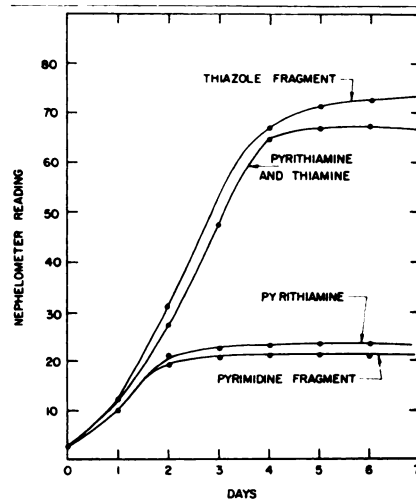
FIGURE 5. Growth of leptospire ICFK in bovine albumin polysorbate-80 glucose medium with the thiazole fragment of thiamine, pyri-thiamine and thiamine, pyrithiamine, and the pyrimidine fragment of thiamine.
