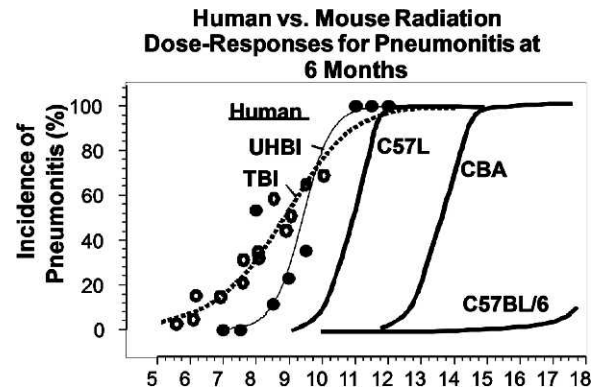
FIG. 1. Radiation dose-responses for severe pneumonitis among humans receiving either single doses of UHBI (●) (117) or single dose-equivalents of TBI (○), most with cyclophosphamide chemotherapy prior to allogeneic bone marrow transplantation (118). These are compared with lethal pneumonitis in three different mouse strains receiving WTL. C57L mice are the most sensitive to radiation and the most comparable to the incidence in humans. CBA mice appear to be more resistant towards radiation pneumonitis. C57BL/6 mice were the most removed from the human data in showing no lethal incidence of pneumonitis over 6 months after lung irradiation.
