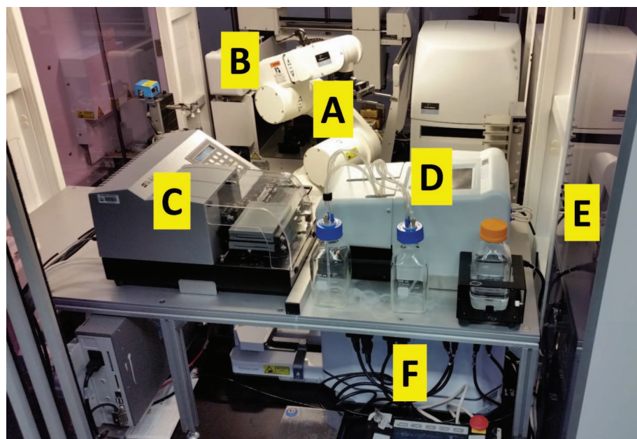
FIG. 2. Layout of the cell::explorer TM at the Columbia Genome Center used as RABiT-II, showing the various subsystems: anthropomorphic robotic arm (A), the JANUS ® liquid-handling system (B), EL406 TM microplate washer (C), the FlexDrop dispenser (D), STX500 automated incubator (E), V-spin TM automated centrifuge (F).
