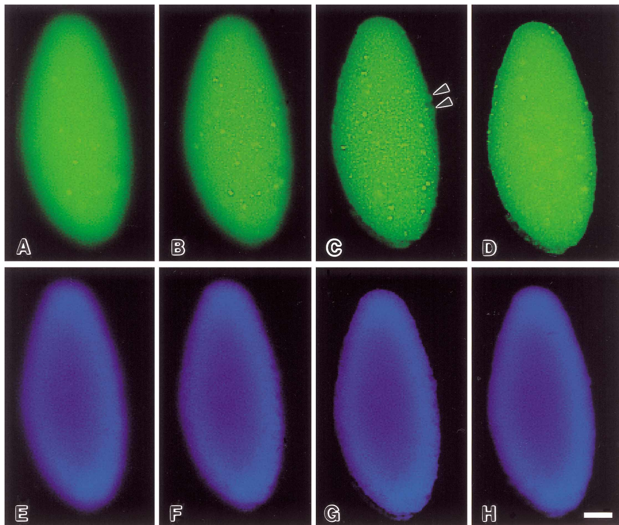
Fig. 1. FISH with Paramecium total genomic DNA probe in Paramecium nuclei. Cell was denatured at 85°C for 10 min in accordance with the conventional method. A–D : FITC images of FISH signals. E–H : corresponding DAPI staining images. A series of optical sections were captured at every 5 steps (2.5 \mu\text{m} ) of z-axis from periphery of the nucleus. All images were deconvoluted to remove the unfocused haze images. Arrow-heads, micronucleus; Bar, 10 \mu\text{m} .
