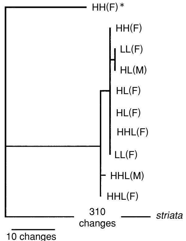
Fig. 2. A maximum parsimony tree of two equally parsimonious topologies obtained by an exhaustive search without character weighting on PAUP* ver. 4.0b (Swofford 1998). Gaps are treated as the fifth character. See Fig. 1 for genome composition of three biotypes. Letters in parentheses indicate male (M) or female (F). A C. hankugensis individual with an asterisk was collected at a different collecting site (Seangcho-myon) from other nine individuals.
