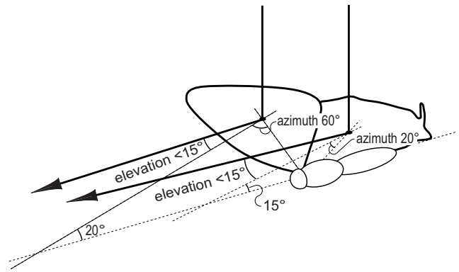
Fig. 6. A schematic illustration of the light course at reflection on the fore- and hind wings of a butterfly in a natural posture. Light from the top is reflected forward at azimuth 60° or 20° by the fore- and hind wings, respectively, and at elevation less than 15°. These azimuths correspond to 20° inward to the body axis in the forewing, and 15° in the hindwing.
