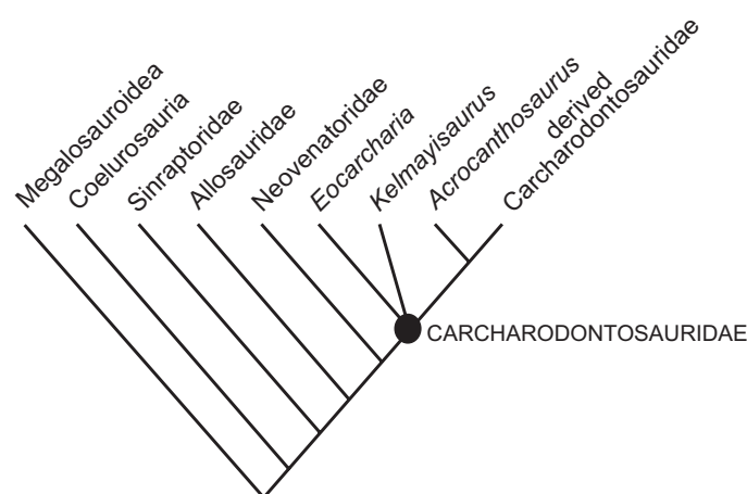
Fig. 3. The phylogenetic relationships of Kelmayisaurus and other basal tetanuran theropods. Strict consensus of 1728 most parsimonious trees (639 steps) recovered by the cladistic analysis (CI = 0.44; RI = 0.64). “Derived carcharodontosaurids” include Shaochilong , Tyrannotitan , Carcharodontosaurus , Giganotosaurus , and Mapusaurus . Kelmayisaurus is recovered as a basal member of Carcharodontosauridae.
