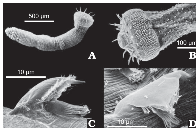
Fig. 6. A modern meiofaunal priapulid worm, Meiopriapulius fijiensis Morse, 1981 from Fiji. A. Overview. B. Detail of the anterior end, illustrating the terminal mouth, the regularly arranged introvert scalids, and the more irregularly arranged trunk scalids. C. Detail of a trunk scalid in lateral view. D. Detail of a trunk scalid in oblique view. Note the presence of marginal teeth, a marginal fringe of hairs, and a midline bundle of hairs, in common with the priapulid scalids from the Kaili microfossil assemblage (cf. Fig. 5A). Images are scanning electron micrographs, reproduced from Morse (1981) with permission of John Wiley and Sons Ltd. and the author.
