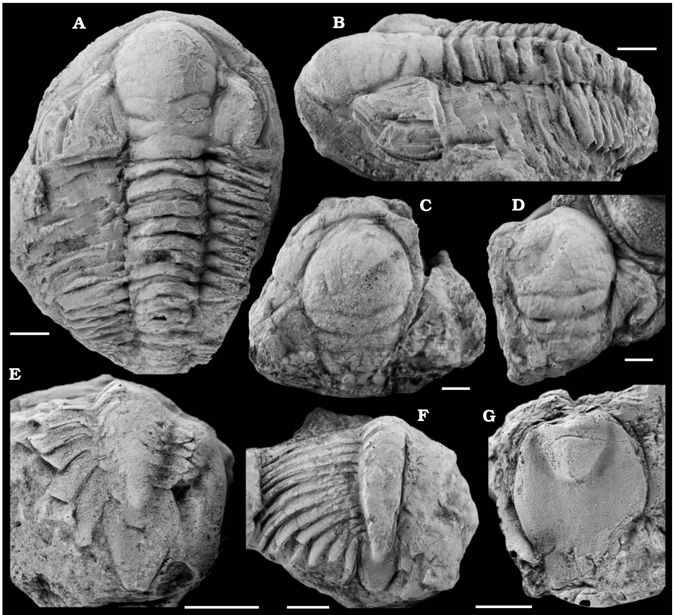
Fig. 7. Paradoxiid trilobite Eccaparadoxides pradoanus (Verneuil and Barrande in Prado et al., 1860) from Sabedo, León province, Solenopleuropsis ribeiroi Biozone, middle Cambrian, Spain. A, B. Lectotypes. A. EM 170 091, fairly complete specimen with two transglabellar glabellar furrow and two weakly incised visible discontinuous furrows. Note convergence of SO and S1, S3, and S4. B. EM 170 091 in lateral view, showing the rear part of the thorax slightly flexed. C–G. Paralectotypes. C. EM 170 092, cranidium with two continuous glabellar furrows and slightly convergent SO and S1. D. EM 170 093, cranidium with two continuous glabellar furrows and two weakly developed discontinuous glabellar furrows. E. EM 170 094, rear part of the thorax with attached pygidium with low spinosity-degree. F. EM 170 095, rear part of the thorax showing large rear pleural spines flanking the pygidium. G. EM 170 096, isolated pygidium. All specimens are photographs taken from internal moulds covered by sublimated \text{NH}_4\text{Cl} . Scale bars 5 mm.
