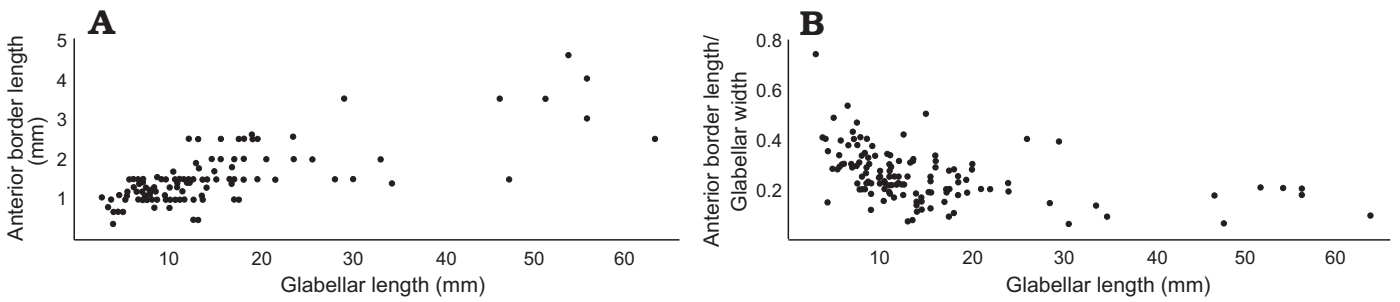
Fig. 15. Bivariate plots showing relationship between glabellar length and anterior border length ( n = 133 ) (A) and anterior border length/glabellar width ratio ( n = 133 ) (B) in paradoxidid trilobite Eccaparadoxides pradoanus (Verneuil and Barrande in Prado et al., 1860) from the Purujosa trilobite assemblage, Solenopleuropsis thoralis Biozone, middle Cambrian, Spain.
