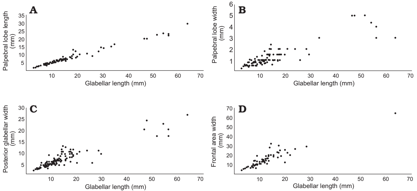
Fig. 16. Bivariate plots showing relationship between glabellar length and palpebral lobe length ( n = 118 ) (A), palpebral lobe width ( n = 101 ) (B), posterior glabellar width ( n = 54 ) (C), and frontal area width ( n = 63 ) (D) in paradoxidid trilobite Eccaparadoxides pradoanus (Verneuil and Barrande in Prado et al., 1860) from the Purujosa trilobite assemblage, Solenopleuropsis thoralis Biozone, middle Cambrian, Spain.
