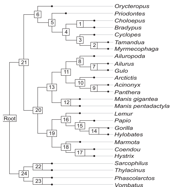
Fig. 4. Phylogenetic tree following Asher and Helgen (2010), as used in the variance decomposition test. The nodes are arbitrarily labeled with numbers.
