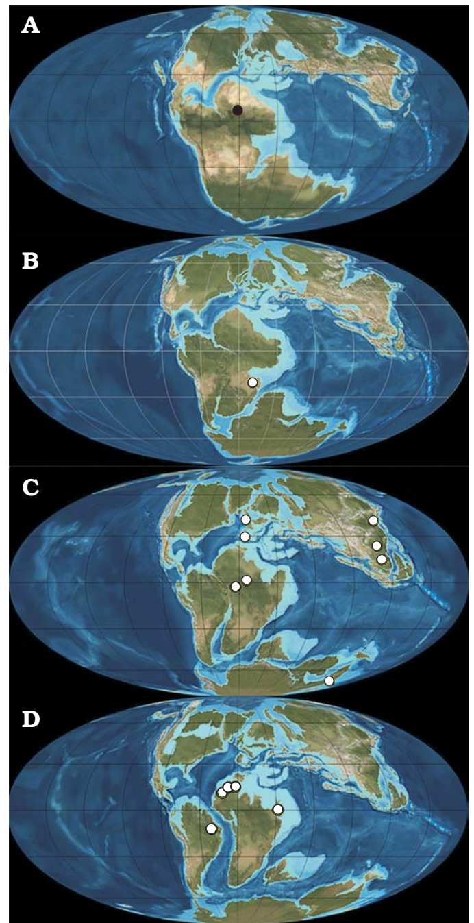
Fig. 6. Generalized palaeogeographic locations of spinosaurids (white) and the specimen of HB site (black), through time from Bajocian–Bathonian (A), Tithonian (B), Barremian–Aptian (C), and Albian–Cenomanian (D). Courtesy of Ron Blakey ( http://jan.ucc.nau.edu/~rcb7/mollglobe.html ), modified and actualized after Bertin (2010).
