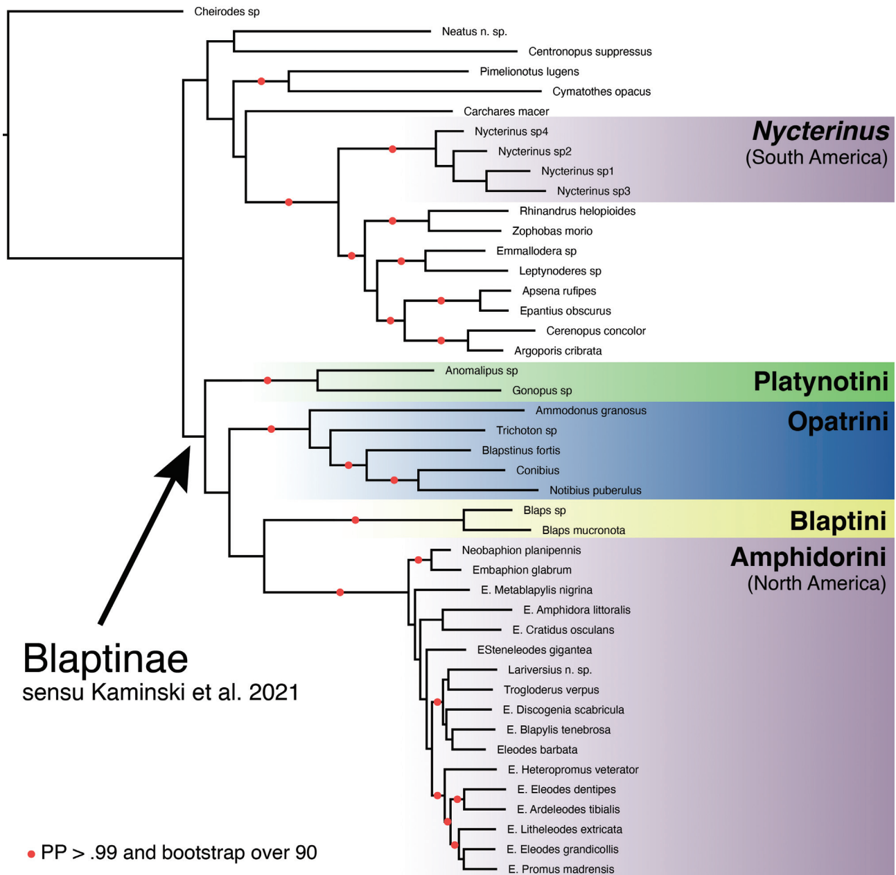
Figure 1. Recovered phylogeny for the Monophyly of Amphidorini dataset. Topology shown corresponds to the maximum likelihood reconstruction highlighting the two unrelated clades of Amphidorini and the three other Blaptinae tribes sampled. Branches marked with a red dot were recovered in both Bayesian inference and maximum likelihood analyses with at least .99 posterior probabilities and 90 bootstrap values, respectively.
