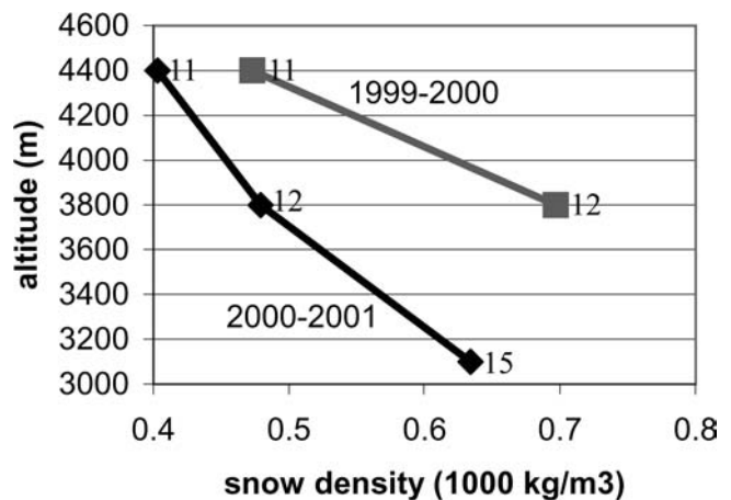
FIGURE 6. Average snow density of the snowpack over two winters prior to onset of the spring melt for Telbrung (3170 m), Sundar (3820 m), and Rambrong (4440 m) for winters 1999–2001. The numbers next to data points refer to station identification numbers in Table 1.
