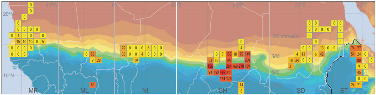
Figure S39. Red-cheeked Cordon-bleu Uraeginthus bengalus ( n/km^2 ).
