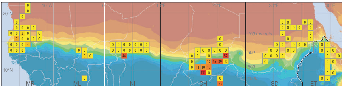
Figure S22. Purple Starling Lamprotornis purpureus ( n/km^2 ).
