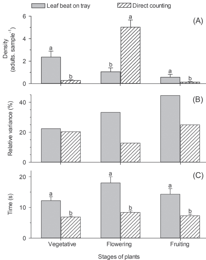
Fig. 2. (A) Adult density of Bemisia tabaci (means ± standard errors), (B) relative variance of densities, and (C) sampling times of Bemisia tabaci adults using direct counting and leaf beating on a white tray methods in melon crops in the vegetative, flowering, and fruiting stages. For each phenological stage, the histograms with lowercase letters indicate significantly different means according to the F test ( P < 0.05 ).
