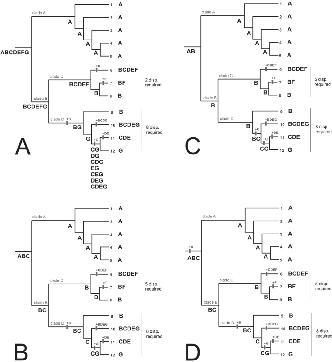
Fig. 6. Event-based analysis by DIVA. A: Scenario 1 (ancient widespread origin) : biogeographic scenario using maxareas = 7, required 10 events of dispersion/dispersal. For the node 11+12 we arbitrarily chose the ancestral distribution CG (Amazon + Atlantic Forest) within the 7 options resulting for the node. B: Scenario 2 (ancient restrict origin) : biogeographic scenario using maxareas = 4, required 13 events of dispersion/dispersal. The basalmost ancestral distribution occurring in ABC (Nearctic + Caribbean + Amazon). C: Scenario 3 (northern origin) : same optimization as Scenario 2, but differing in the basalmost ancestral distribution restricted to AB (Nearctic + Caribbean). D: Scenario 4 (southern origin) : same optimization as Scenario 2, but including an additional event in the cladogram root unlikely to be inferred by DIVA: the dispersal of the ancestral occurring from BC to A, then becoming ABC. Total events required is 14. (Legends: numbers refers to species of Heterostylum ; letters refers to areas: A, Nearctic; B, Caribbean; C, Amazon forest; D, Cerrado; E, Caatinga; F, Chado; G, Atlantic forest. For Scenarios 2, 3 and 4, DIVA analyses optimized alternative distributions for some nodes; please see the Supplementary Material)
