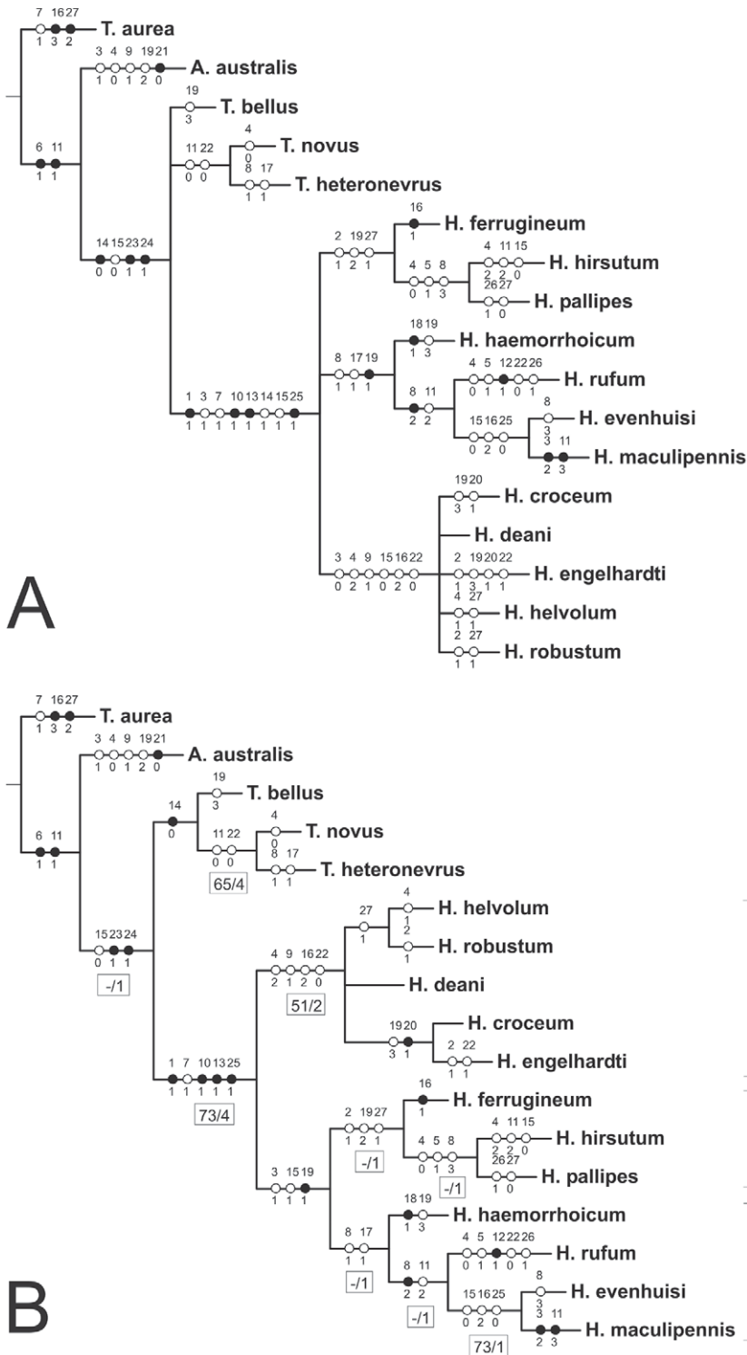
Fig. 1. A: Consensus tree of 6 most parsimonious trees resulting from equal weighting analysis, under acctrans optimization (length = 74 steps, CI = 0.51, RI = 0.57). B: Single most parsimonious tree resulting from successive weighting analysis, under acctrans optimization (length = 68 steps, CI = 0.55, RI = 0.64). Black circles represent unique changes; white circles represent multiple changes. Bootstrap values and Bremer support values are shown inside rectangles below branches, separated by “/”.
