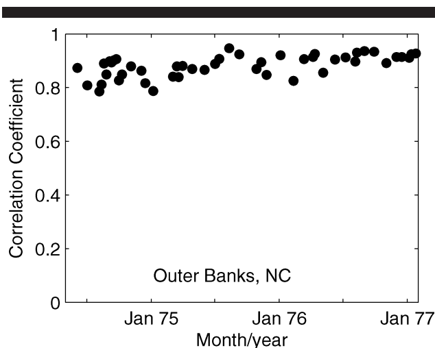
Figure 13. Correlation coefficients between along-coast variability in shoreline change and along-coast variability in subaerial volume change for each survey date for the Outer Banks of North Carolina.
