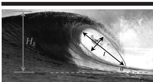
Figure 4. Wave breaker intensity ( B_r ) defined by the vortex ratio of w to l (after Mead and Black, 2001c).
