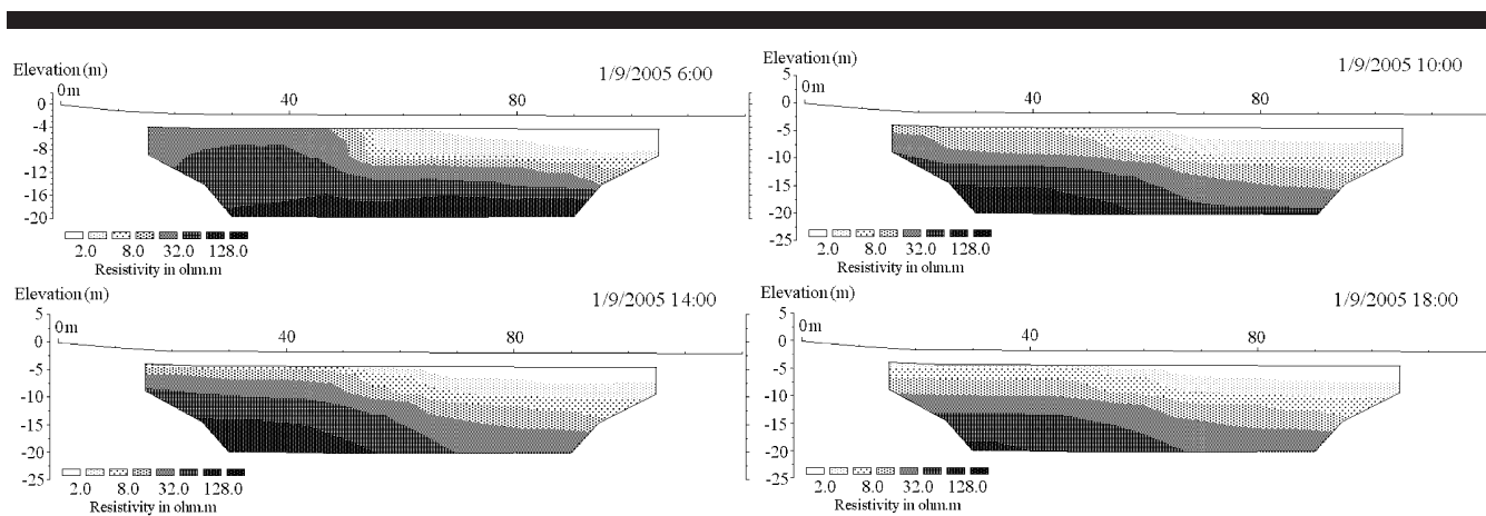
Figure 3. Temporal changes in resistivity from low tide (top left; 0600, 9 January 2005) to high tide (bottom right; 1800, 9 January 2005). Dark colors are freshwater and light colors are saline water.
