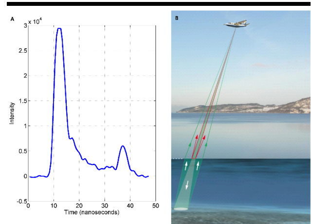
Figure 1. (A) Example of the Chiroptera II green laser waveform showing the large return from the sea surface and smaller return from the seabed. (B) Schematic of the Chiroptera II green and NIR lasers' interaction with the sea surface and seabed (adapted from Leica AHAB).
