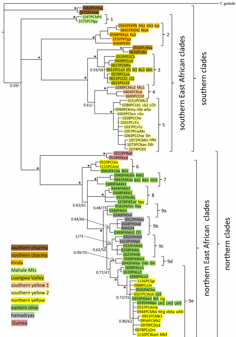
Figure 3. Bayesian phylogram of Papio cyt b haplotypes (Bayesian tree reconstruction for identification of clades) (* Bayesian posterior probabilities > 0.95, ML bootstrap support values >75%). Tip labels refer to the species (as identified by phenotypic characters; PA = P. anubis ; PC = P. cynocephalus ; PH = P. hamadryas ; PK = P. kindae ; PP = P. papio ; PU = P. ursinus ) together with the sampling location. Several haplotypes were found at more than one site. This is indicated by the listing of more than one site abbreviation at some branch tips.
