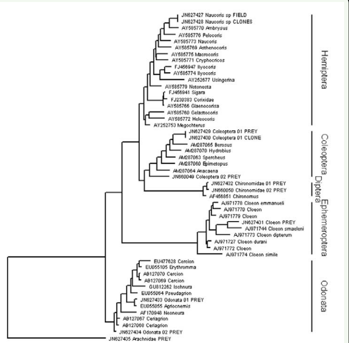
Figure 2. Maximum likelihood rrnL gene tree reconstructed using a GTR model of evolution, including newly sequenced Naucoris sp. (terminals labeled FIELD), potential prey (PREY), cloned PCR products from Naucoris sp. guts / mouthparts (CLONES), and highly ranked sequences according to blastn queries (with GenBank alphanumeric accession codes, see text for criteria). High quality figures are available online.
