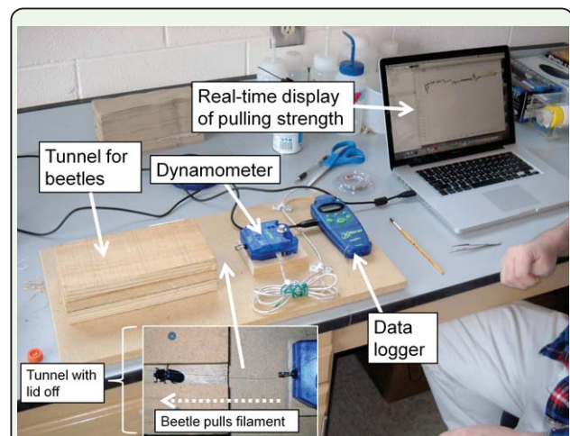
Figure 1. Apparatus for measuring pulling force of Odontotaenius disjunctus . The beetles were tied to a dynamometer with nylon thread and allowed to walk in a wooden tunnel (inset photo). A data-logger recorded the pulling force over a 10 min period, which was graphed in real-time on the computer (see Figure 2). High quality figures are available online.
