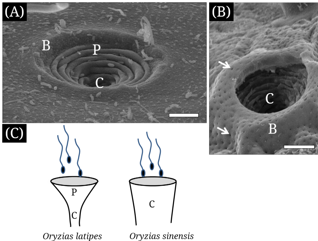
Fig. 3. Scanning electron micrographs showing types of micropyle in Oryzias latipes (funnel shape with a pit – A) and O. sinensis (conical shape without a pit – B). C is a schematic diagram of different micropyles. Arrow – pore canal, B – boundary part, C – micropyle canal, P – micropyle pit. All bars indicate 5 \mu\text{m} .
