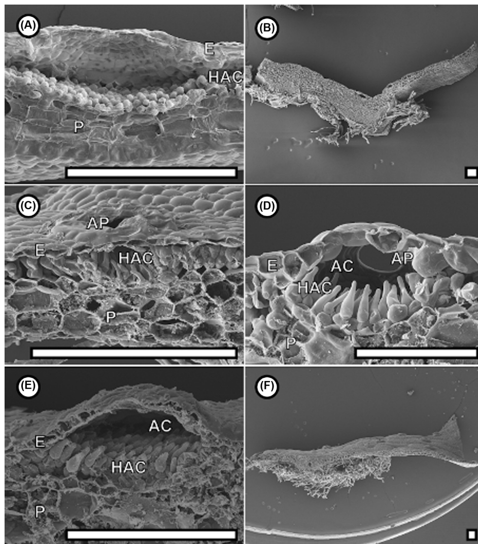
Figure 3. Cross sections of freshly (A–D) and frozen (E–F) dried C. salebrosum (SEM). AC: air chamber; AP: air pores; E: epidermis; HAC: hyaline apical cell; P: parenchyma. Scale bars: 200 µm.
