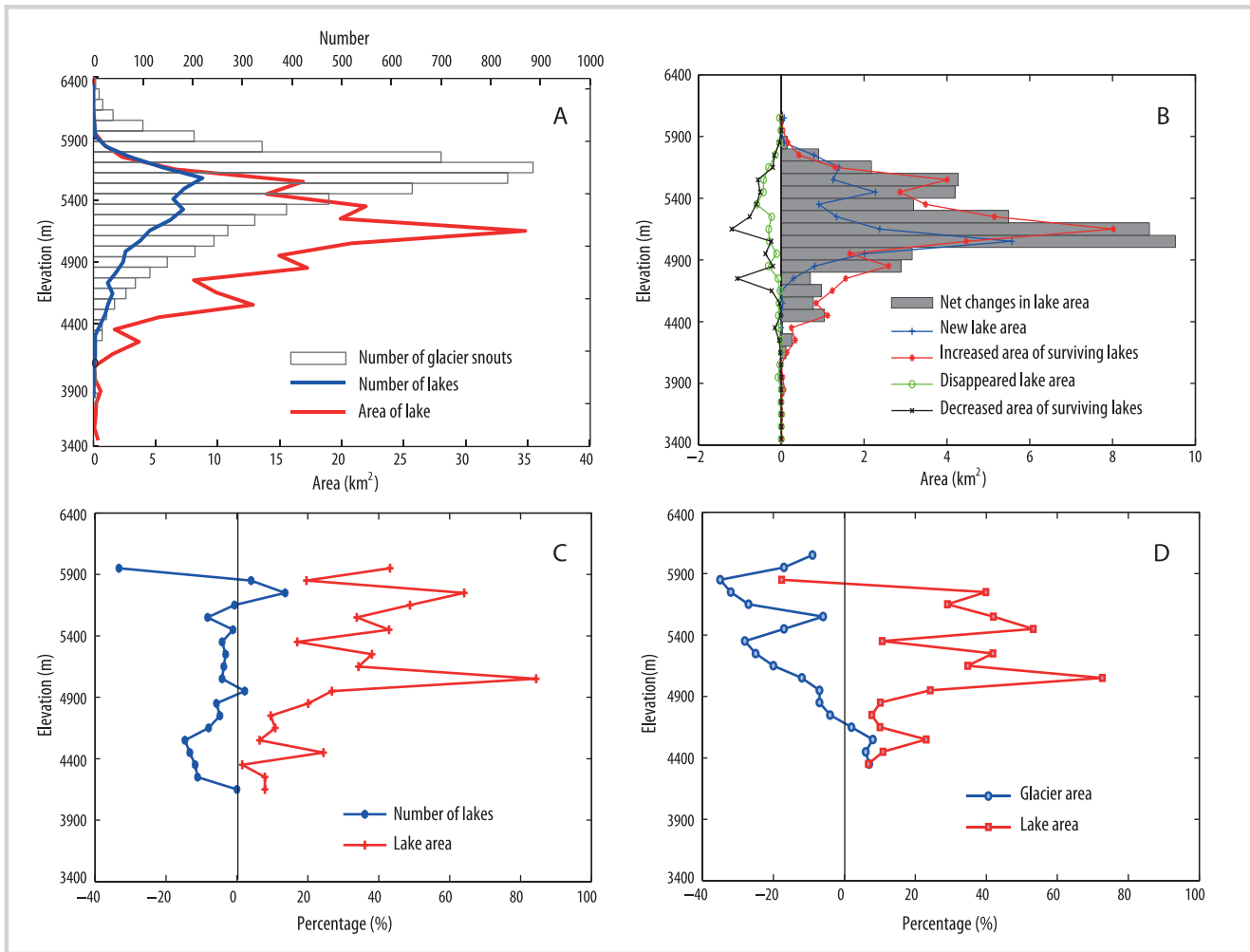
FIGURE 3 Distributions and changes of glacial lakes in the Chinese Himalaya, organized in 100-m elevation bands over the past 30 years. (A) Distributions of lake area, number, and glacier snout number; (B) area variations of surviving lake, new lake, disappeared lake area, and net changes; (C) lake changes in percentages over the past 30 years (only 100-m elevation bands with more than 10 lakes are shown); (D) contrasted area changes of glacier and lake in Mt Qomolangma National Natural Preserve Region.
