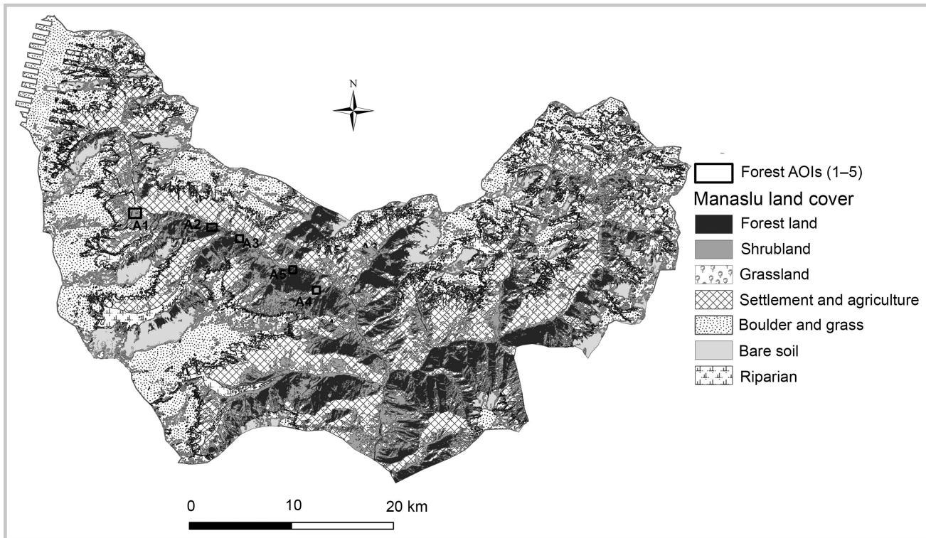
FIGURE 3 MCA land cover classification and forest AOs. (Data source: U.S. Geological Survey Landsat 5 TM, October 2009, 30-m resolution and ICIMOD MCA shape file; map by Janardan Mainali and John All.)
