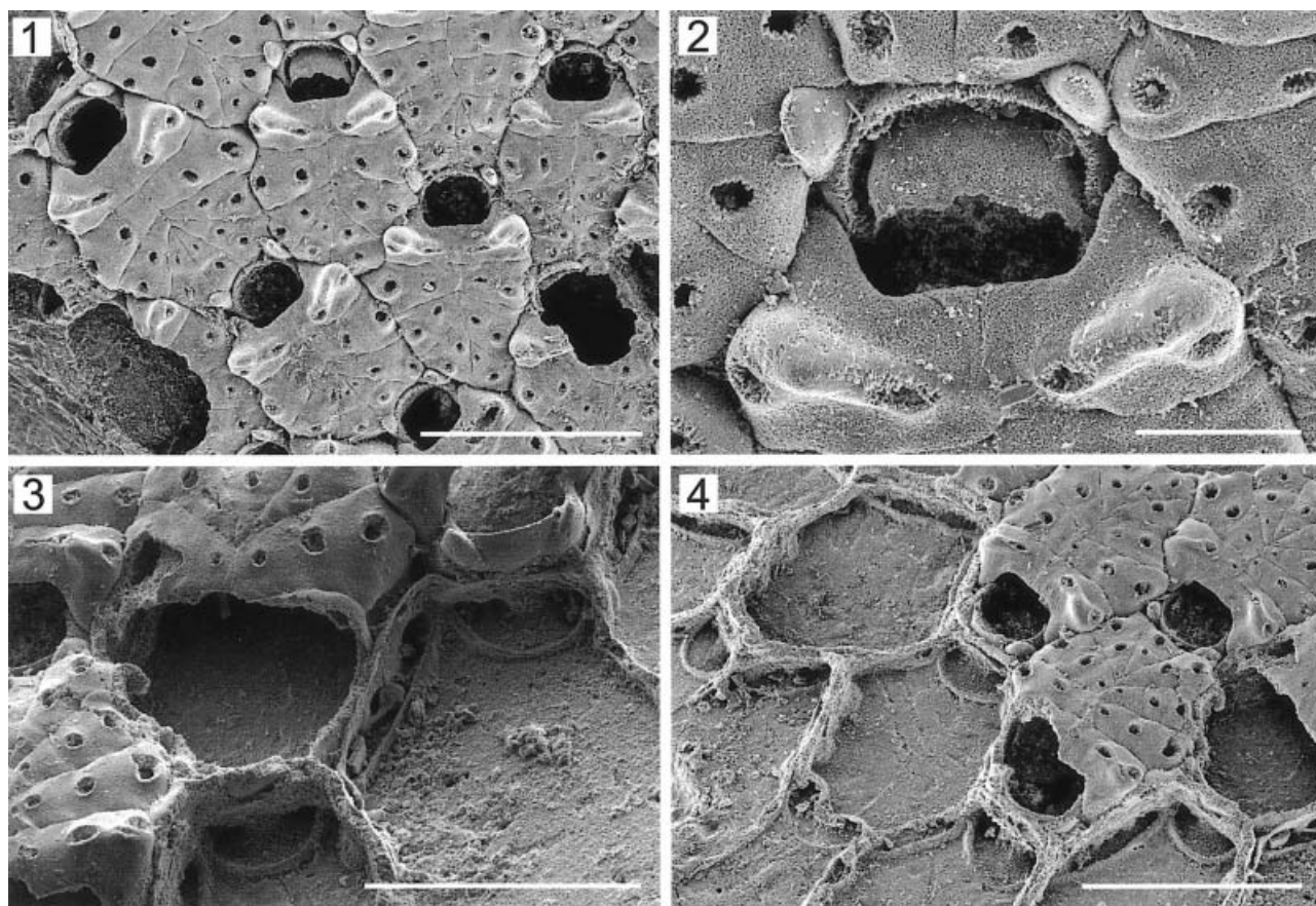
Figure 3. Hayamiellina constans sp. nov. ZIHU-2319, late Middle Miocene, southwestern Hokkaido, Japan. 1. Ephebic autozooids. Note the conspicuous crests on the suboral costae. 2. Close-up of orifice. Note the distolateral tubercles. Debris occupies the orifice. 3. Colony margin showing distal and lateral pore-chambers. 4. Same, another part of colony. 1, 4, scale bar = 500 \mu\text{m} . 2, scale bar = 100 \mu\text{m} . 3, scale bar = 400 \mu\text{m} .
