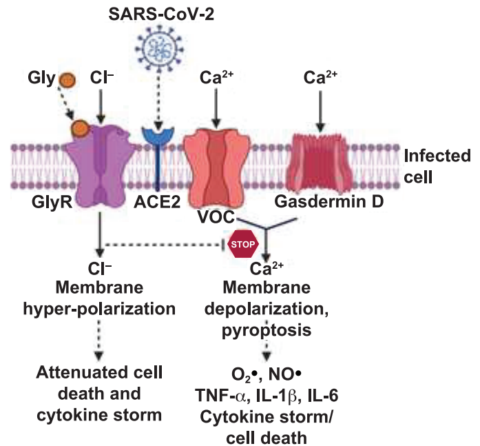
FIG. 1. A hypothetical mechanism of how glycine may reduce SARS-CoV-2-mediated tissue damage and cytokine storm. SARS-CoV-2 can infect target cells through the ACE2 protein. The infection may cause cell death through pyroptosis, which requires calcium influxes from voltage-operated calcium channel (VOC) or gasdermin D pores and ensuing cellular membrane depolarization, free radical generation and secretion of pro-inflammatory cytokines. Glycine, by binding its receptor GlyR, induces a chloride influx that causes cellular membrane hyperpolarization that protects the cells from pyroptosis and proinflammatory cytokine secretion.
