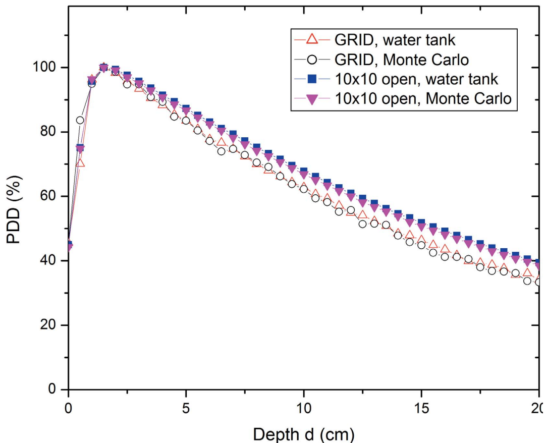
FIG. 4. Percentage depth-dose curves of a 10 \times 10 \text{ cm}^2 open field and a 10 \times 10 \text{ cm}^2 GRID field. The PDD of the GRID field is measured by water tank and calculated using the Monte Carlo technique (29).
