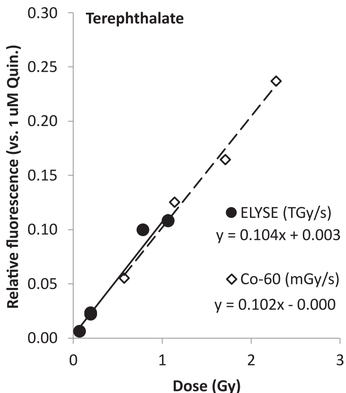
FIG. 9. Comparison of the fluorescence of liquid samples of the terephthalate dosimeter (0.1 mM terephthalic acid in 0.4 M NaOH) caused by irradiation with picosecond electrons from ELYSE and with ^{60}\text{Co} gamma-ray source; the dose was determined by Fricke dosimetry (see text); the liquid fluorescence measurement was normalized against the fluorescence of solutions of 1\ \mu\text{M} quinine in 0.4 M \text{H}_2\text{SO}_4 (for more details see Supplementary Information; https://doi.org/10.1667/RADE-20-00292.1.S1 ).
