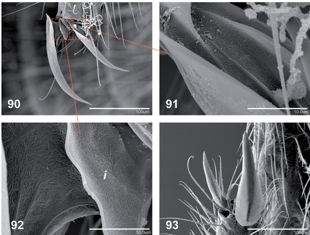
Figs 90-93. Plusiocampa (Venetocampa) pirnati Sendra & Borko, sp. nov. (90) Pretarsus of metathoracic leg, lateral view. (91) Detail of proximal portion of anterior claw in lateral view. (92) Detail of intermediate structure between claws ( i = intermediate sheet). (93) Pretarsus of metathoracic leg, dorsal view.
