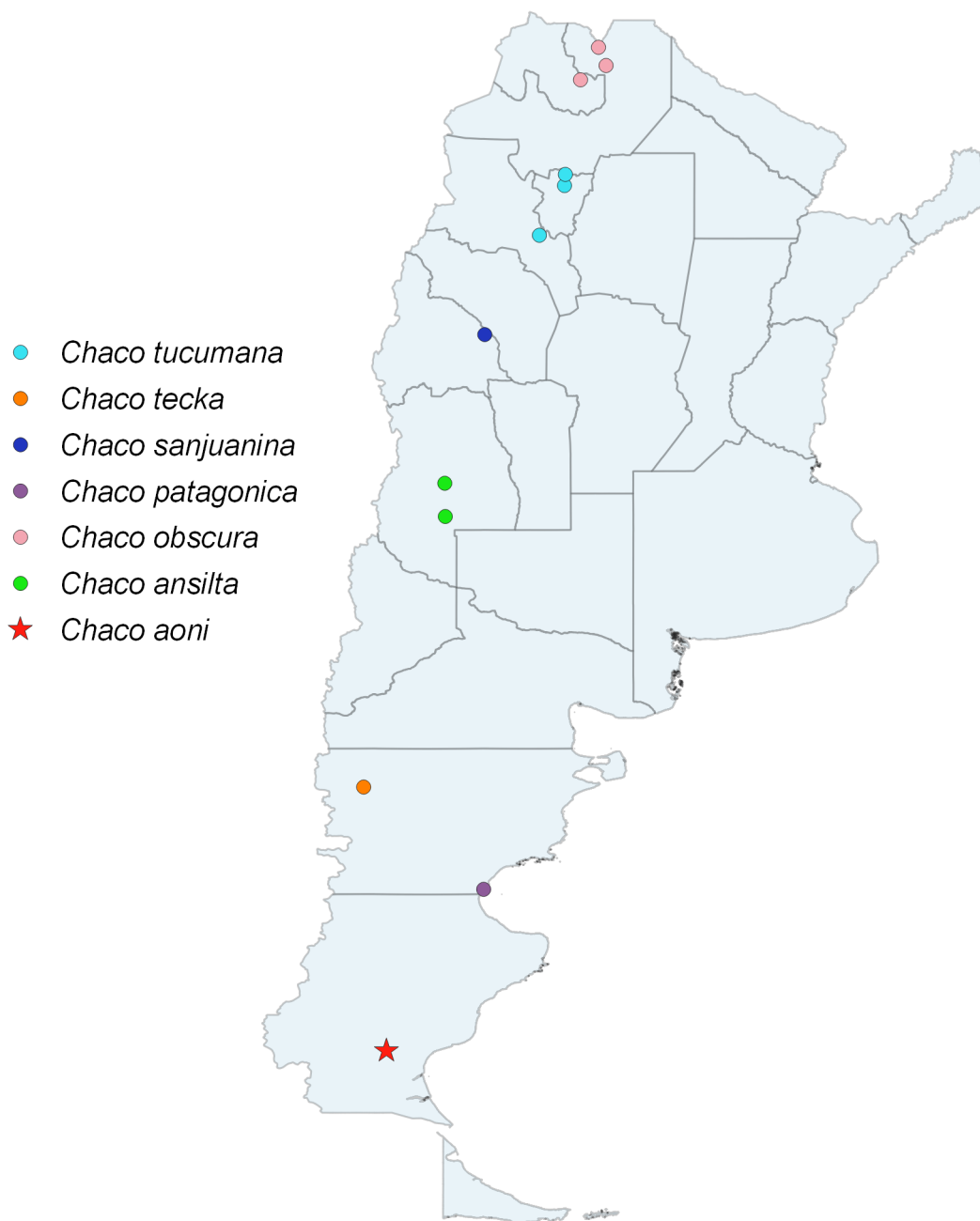
Fig. 7. Locality map of the known species of Chaco in Argentina.
