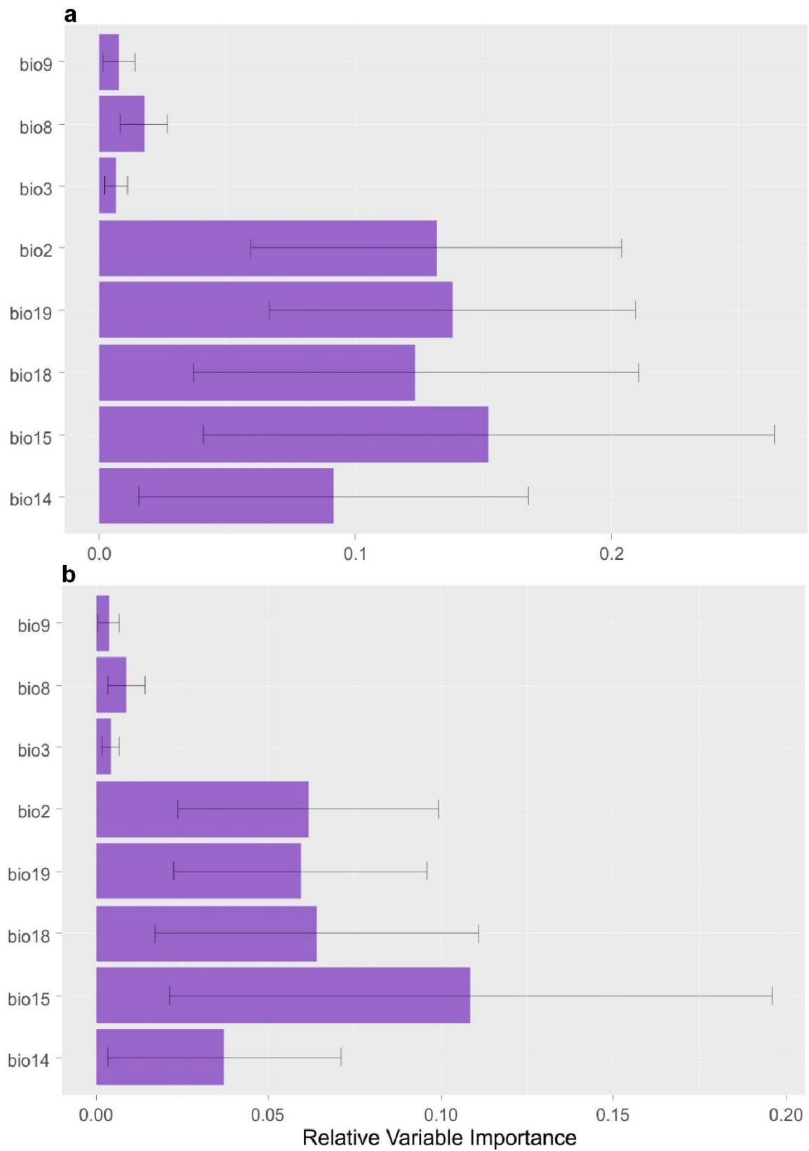
Figure S2.—Relative importance of variables based on exclusion from model relative to being included (a), and correlating the predicted values to values predicted when a variable is randomly permuted (b).
