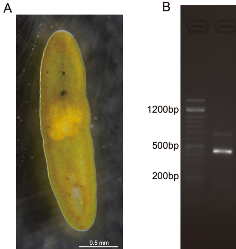
Supplementary Figure S1. Image of Praesagittifera naikaiensis and PCR products using primers mICOLintF/HCO2198 and P. naikaiensis gDNA. (A) A mature adult of P. naikaiensis . Yellow eggs are observed in the center of body. (B) Electrophoresis of the products of PCR using primers mICOLintF/HCO2198 and P. naikaiensis gDNA. PCR products were observed at the expected position in the gel image (367 bp).
