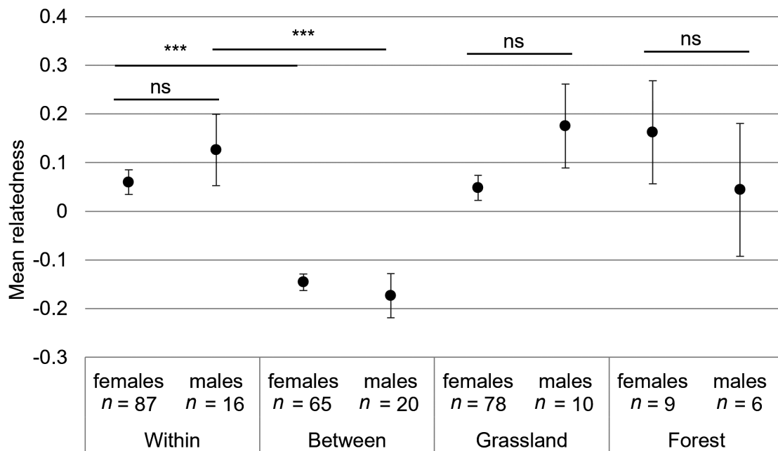
Supplementary Figure S2. Mean relatedness of Japanese serow among sexes within areas and between areas in grassland and forest areas at Mt. Asama. n : number of pairs of individuals, ns: no significant difference ( P > 0.05 ), ***: P < 0.001 .
