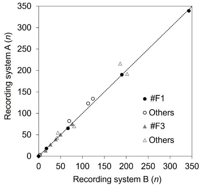
Supplementary Fig. S1. Comparison of the number of pulsed call sequences between recording systems A and B. The number of Type-1 sequences for #F1 and that of all sequences for the conspecifics are represented by closed and open black circles, respectively. The number of Type-1 sequences for #F3 and that of all sequences for her conspecifics are represented by closed and open grey triangles, respectively. The dotted line is straight with a slope of 1.0.
