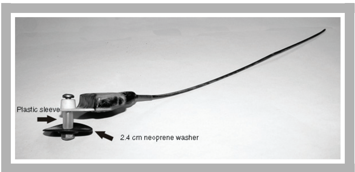
Figure 2. Modified ear-tag transmitter with plastic sleeve and neoprene washer design.
