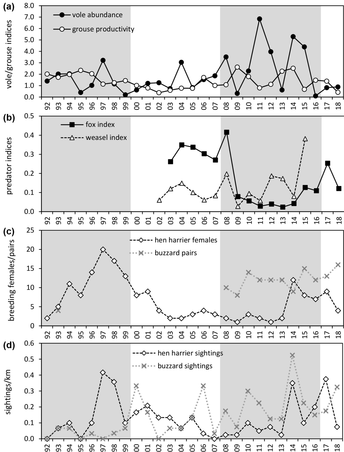
Figure 2. Annual indices of (a) field vole abundance (voles 100 trap nights -1 ) and red grouse productivity (young adult -1 ), (b) mammalian predator abundance (fox: scats/km/day×10; weasel: proportion of tunnels with footprints), (c) number of breeding hen harriers and buzzards and (d) hen harrier and buzzards sighting rates during breeding bird surveys, on Langholm Moor between 1992 and 2018. Periods of active grouse moor management (1992–1999 and 2008–2016) are highlighted in grey (note that predator abundance indices in 2008 were assigned to the unmanaged period for analyses). Foxes and weasels were culled when the moor was managed for grouse, whilst raptors were protected in all years.
