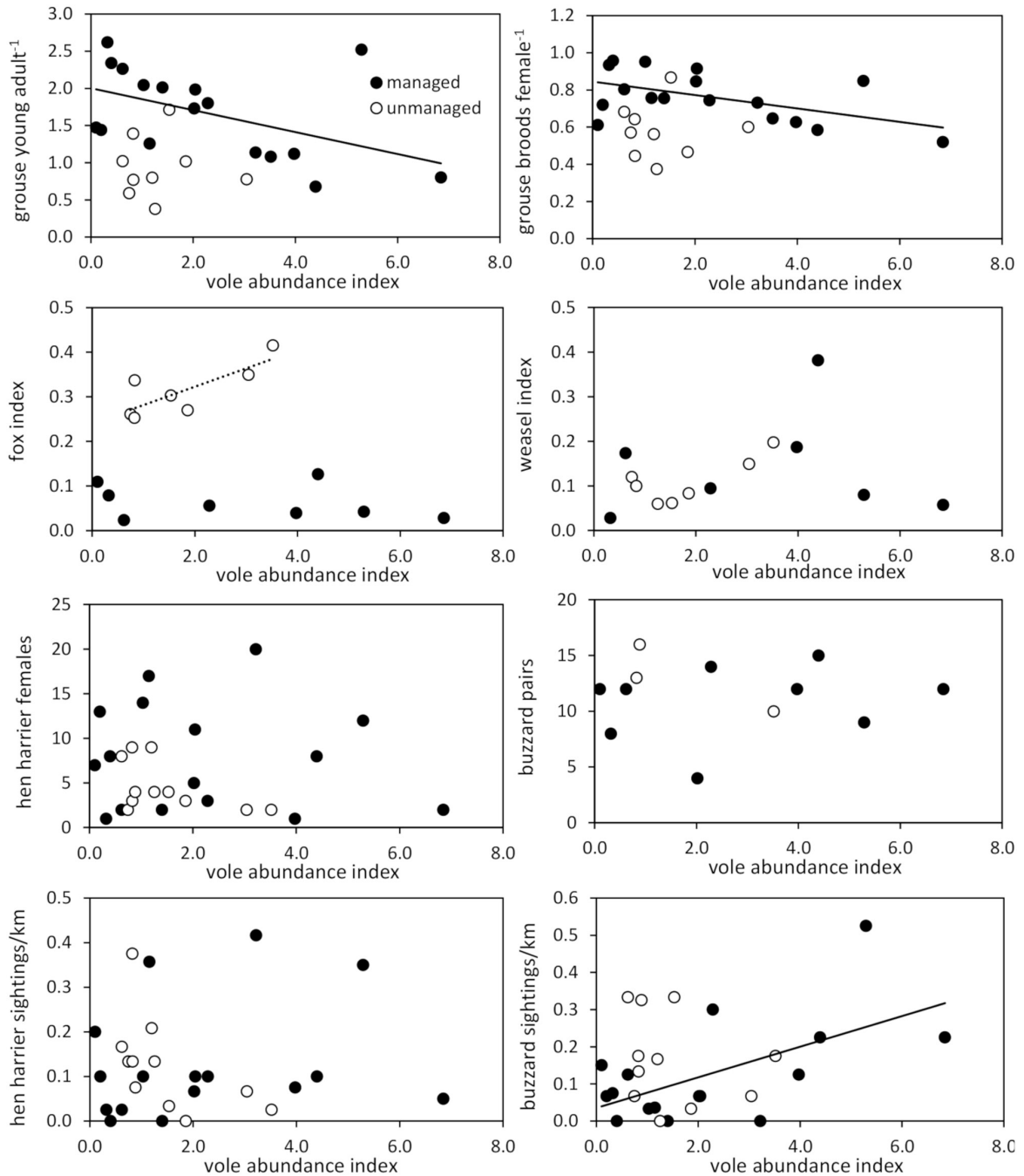
Figure 3. Relationships between field vole abundance (voles 100 trap nights -1 ) and indices of red grouse productivity, abundance of mammalian predators (fox index: scats/km/day \times 10; weasel index: proportion of tunnels with footprints) and abundance of raptors in managed (filled circles) and unmanaged (open circles) periods. Trend lines are only shown for significant relationships (solid line: overall relationship irrespective of management; dotted line: relationship during unmanaged years only).
