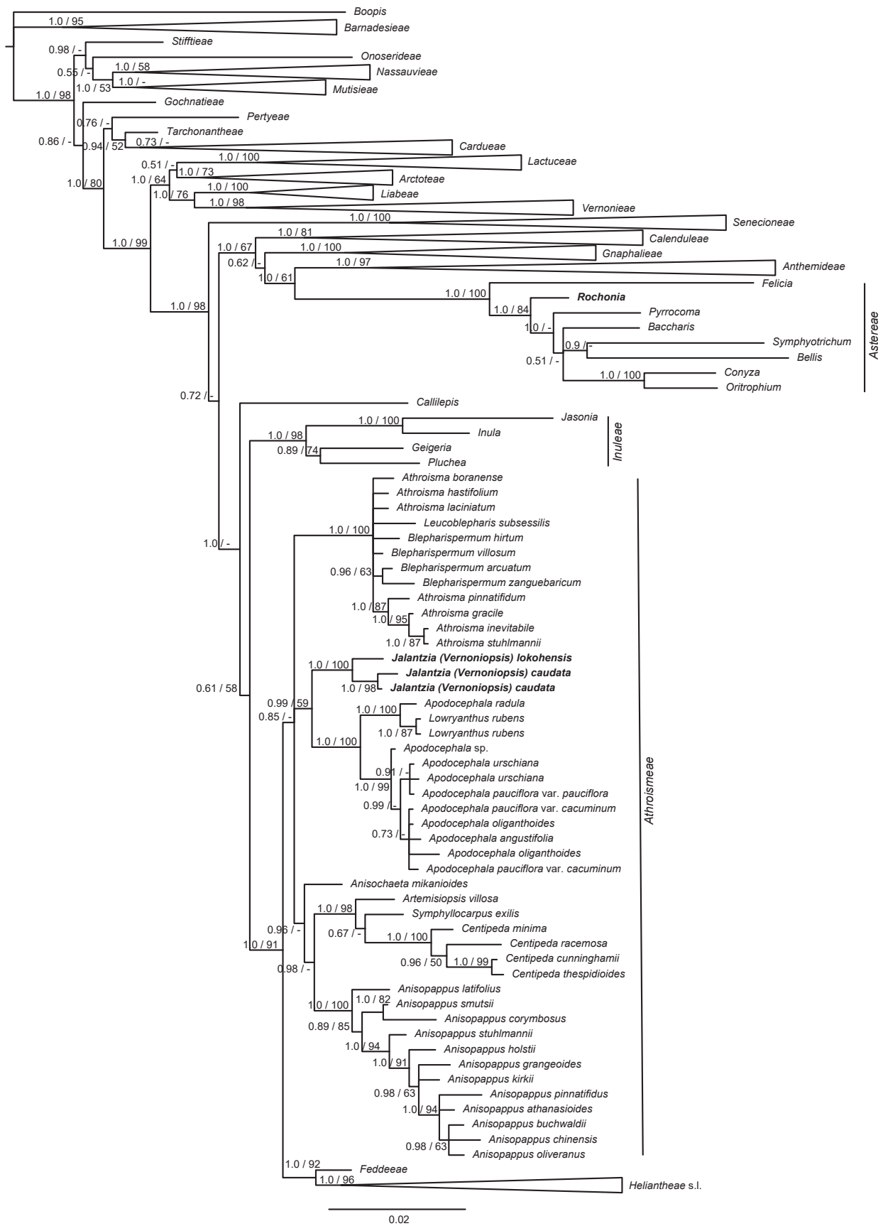
Fig. 2. Bayesian fifty-percent majority-rule consensus tree from an analysis of the Asteraceae ndhF dataset, showing position of Rochonia within Asteroideae and Jalantzia (Vernoniopsis) within Athroismeae . Numbers above branches indicate posterior probability (PP) and bootstrap values (BS), bootstrap values <50 are indicated by a dash. Scale bar shows number of substitutions per site.
