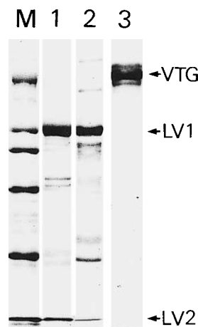
Fig. 21. SDS-PAGE showing the cleavage of the VTG by cathepsin D. Purified VTG (4 \mu g protein) was incubated with quail liver cathepsin D (50 ng protein) for 1 day at 37°C, electrophoresed and stained with Coomassie brilliant blue (lane 2). Lane 1, yolk proteins; lane 3, VTG. M, marker proteins of 200, 116, 97, 66, 45 and 31 kD from top to bottom; LV1 and 2, lipovitellin 1 and 2.
